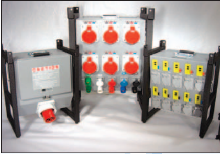
Pin & Sleeve Distribution Center with Edison GFCI Distribution
